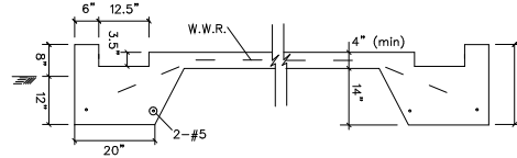
SEC B-B
