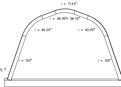
ARCH PROFILE
