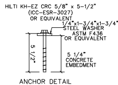
ANCHOR DETAIL
