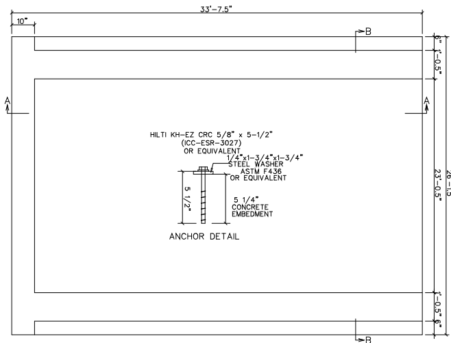
FOUNDATION PLAN
