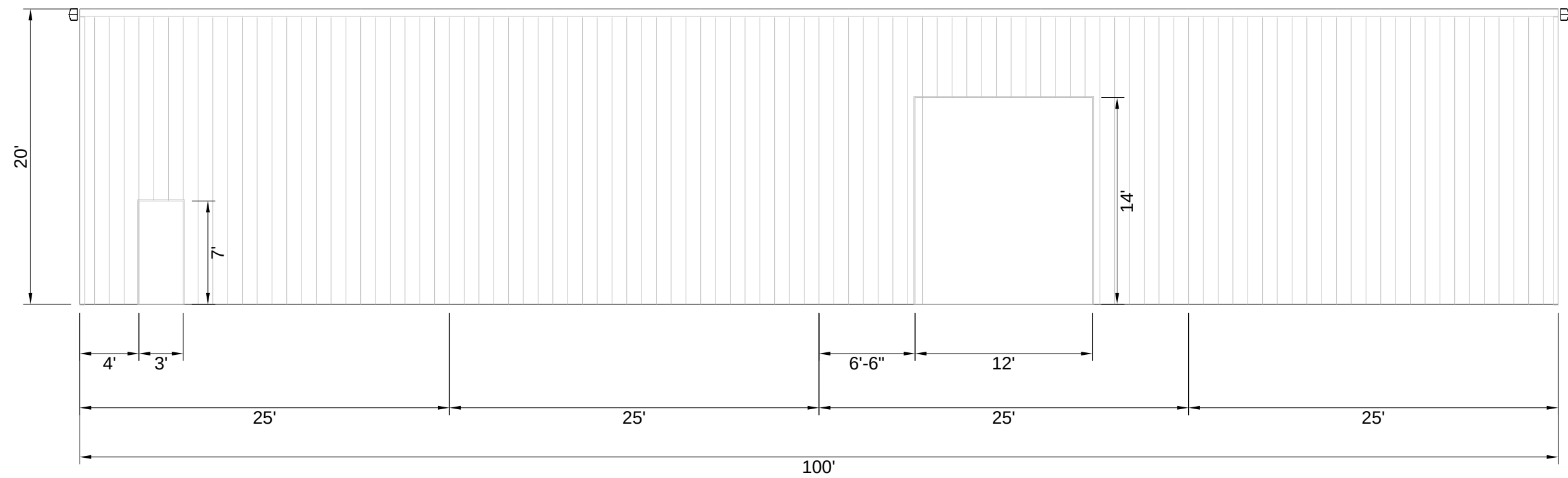
Front Wall
