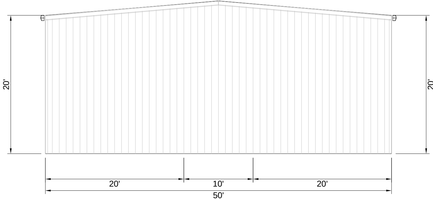
Right Wall
