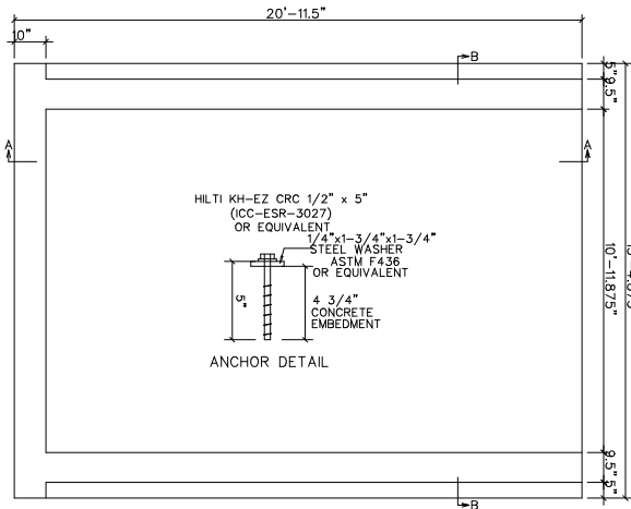
FOUNDATION PLAN
